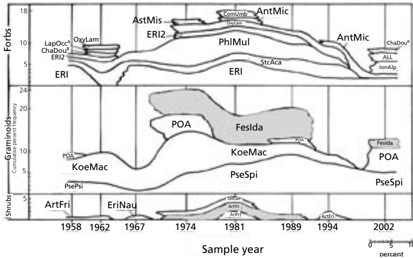
Figure 5 (top). Facies diagram for MC1T1, outside Blacktail enclosure (grazed area), Yellowstone National Park. Sample years are at vertical lines. Intervals between samples were manually interpolated. Percent cumulative frequency is diagrammed to scale by lifeform. A= annual; B= biennial. Species abbreviations are listed in Appendix A.
